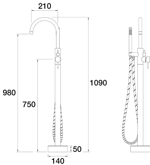
Lugano Floor Bath Filler Mixer with Handshower Gooseneck A22.075.1.41 - Brushed Brass
