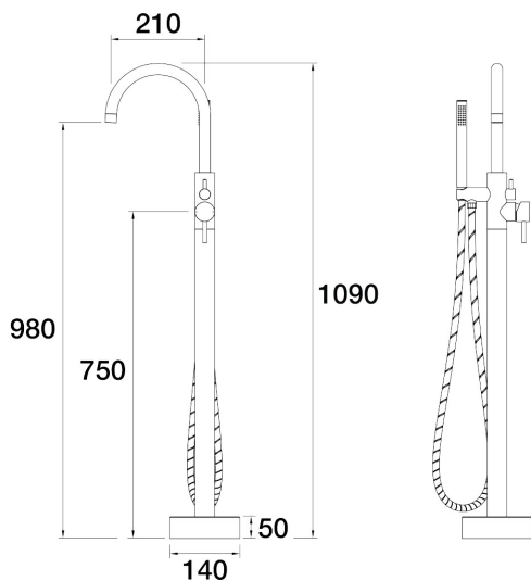
Lugano Floor Bath Filler Mixer with Handshower Gooseneck A22.075.1.45 - Native Brass
