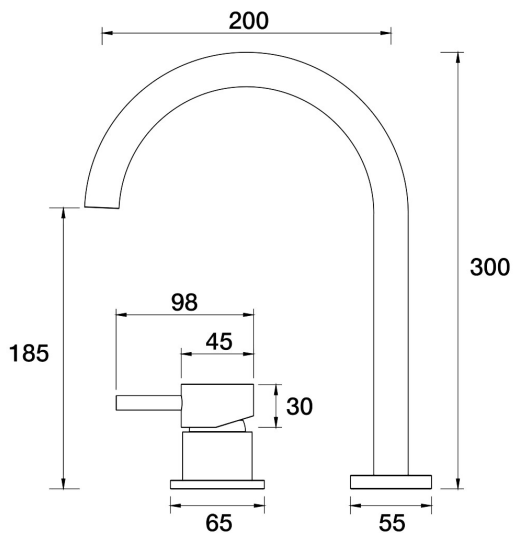
Lugano Hob Mixer with Gooseneck Outlet A22.081.2.12 - 23k Brushed Gold
