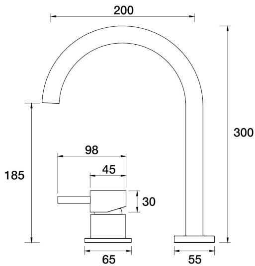
Lugano Hob Mixer with Gooseneck Outlet A22.081.2.45 - Native Brass
