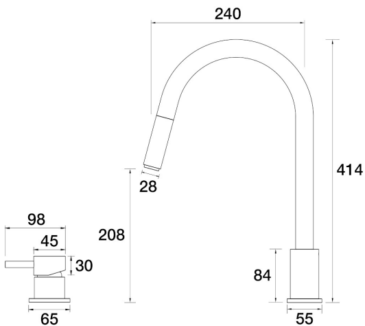
Lugano Hob Mixer with Gooseneck Pullout Outlet A22.081.3.34 - Matt Black
