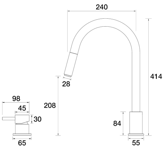
Lugano Hob Mixer with Gooseneck Pullout Outlet A22.081.3.67 - Vintage Brass
