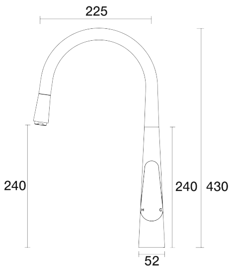
Lava Sink Pull out Mixer A23.022.1.01 - Chrome
