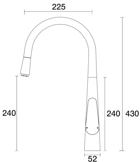
Lava Sink Pull out Mixer A23.022.1.27 - Satin Pearl
