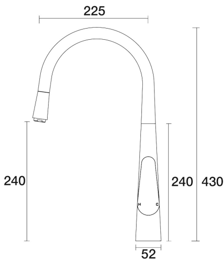
Lava Sink Pull out Mixer A23.022.1.48 - Copper
