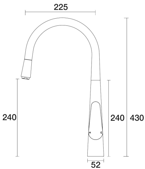
Lava Sink Pull out Mixer A23.022.1.52 - Burnished
