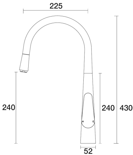
Lava Sink Pull out Mixer A23.022.1.67 - Vintage Brass
