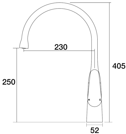
Lava Sink Dome Mixer A23.023.1.45 - Native Brass
