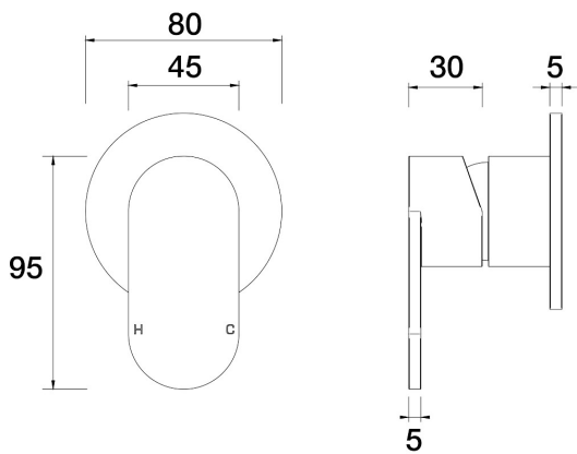
Lava Wall Mixer Shower A23.031.1.67 - Vintage Brass
