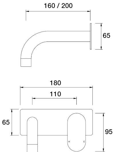
Lava Wall Mixer Basin Set 160mm outlet Incl. plate A23.032.2.01 - Chrome
