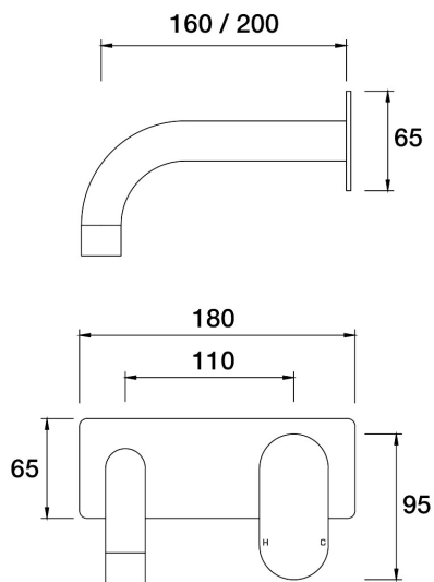
Lava Wall Mixer Basin Set 160mm outlet Incl. plate A23.032.2.48 - Copper
