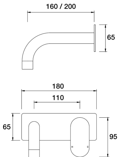
Lava Wall Mixer Basin Set 160mm outlet Incl. plate A23.032.2.52 - Burnished
