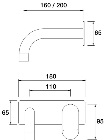
Lava Wall Bath Mixer Set 200mm outlet Incl. plate A23.041.2.40 - Rumbled Brass
