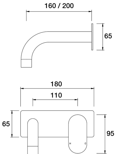
Lava Wall Bath Mixer Set 200mm outlet Incl. plate A23.041.2.57 - Matt Nickel
