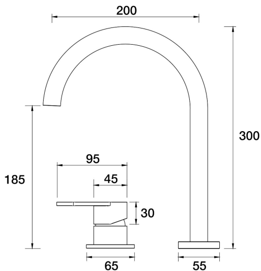
Lava Hob Mixer Set A23.081.2.02 - Brushed Chrome
