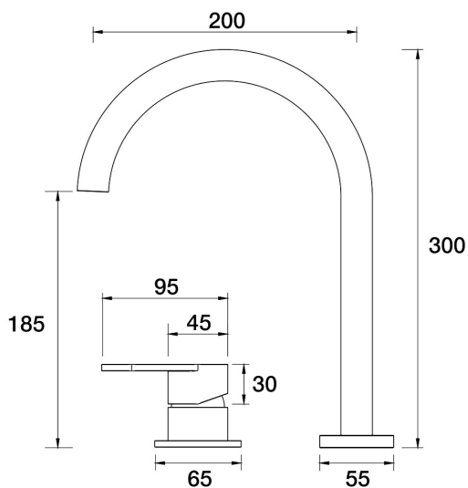
Lava Hob Mixer Set A23.081.2.23 - Gunmetal
