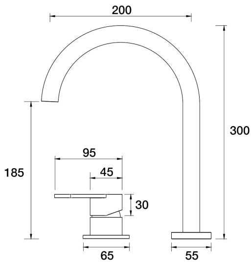
Lava Hob Mixer Set A23.081.2.54 - Volcanic Grey
