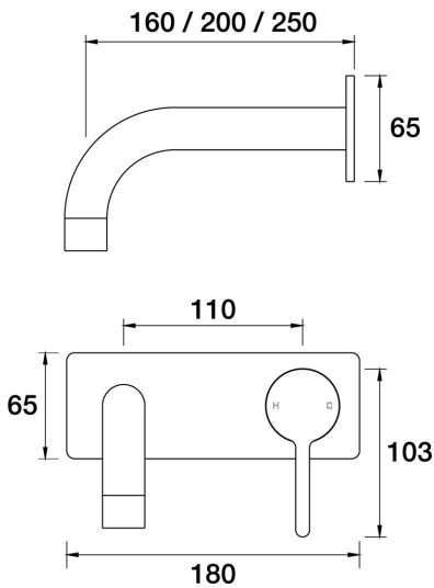
Fuze Wall Mixer Basin Set 200mm outlet Incl. plate A25.032.1.01 - Chrome
