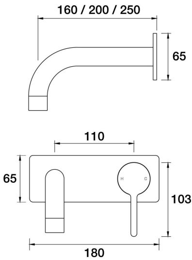
Fuze Wall Mixer Basin Set on plate 250mm A25.032.3.01 - Chrome
