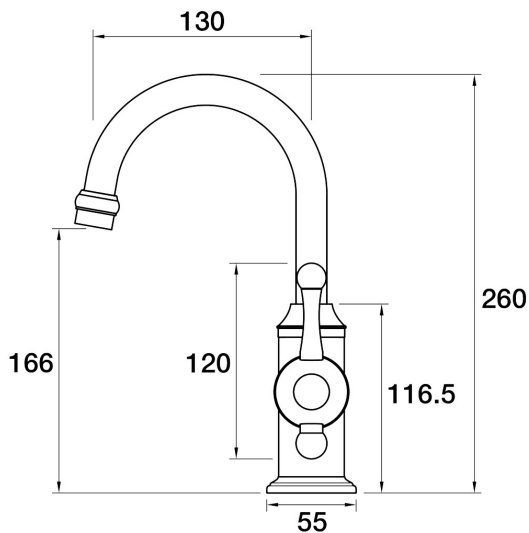
Tudor Hob Basin Mixer A31.011.1.24 - Brushed Gunmetal
