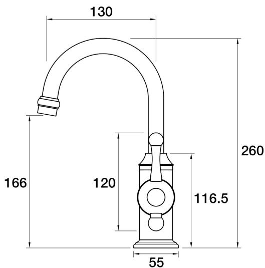
Tudor Hob Basin Mixer A31.011.1.34 - Matt Black
