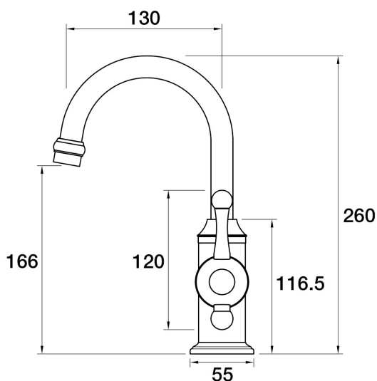
Tudor Hob Basin Mixer A31.011.1.47 - Luminick
