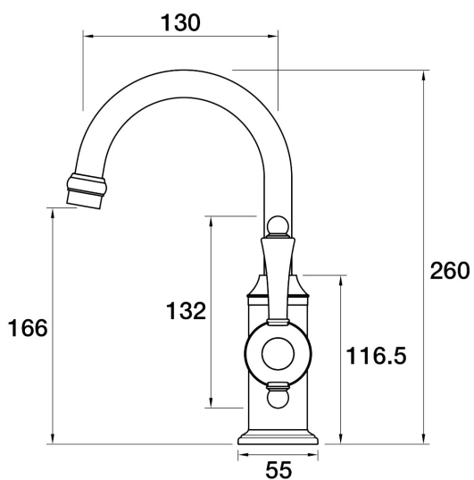
Tudor Hob Basin Mixer Porcelain Handle A31.011.2.02 - Brushed Chrome
