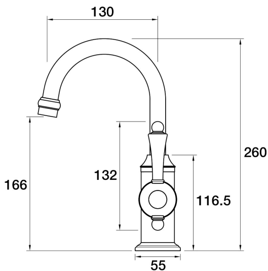
Tudor Hob Basin Mixer Porcelain Handle A31.011.2.41 - Brushed Brass
