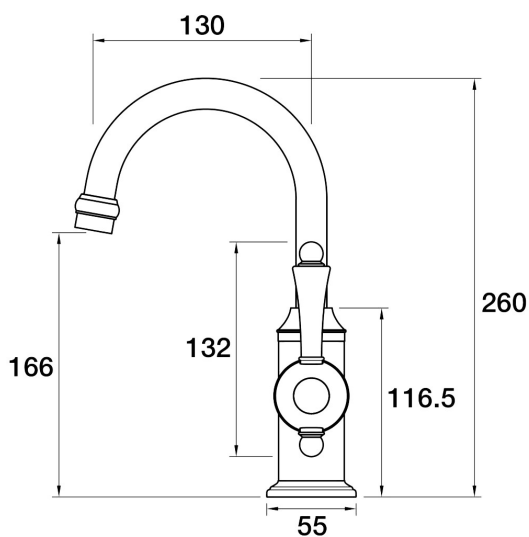
Tudor Hob Basin Mixer Porcelain Handle A31.011.2.52 - Burnished
