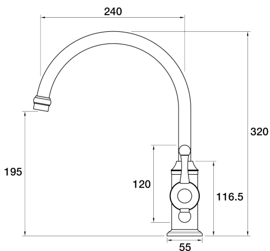
Tudor Sink Mixer A31.021.1.43 - Brass
