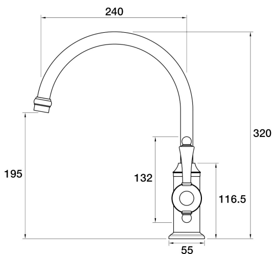
Tudor Sink Mixer Porcelain Handle A31.021.2.02 - Brushed Chrome
