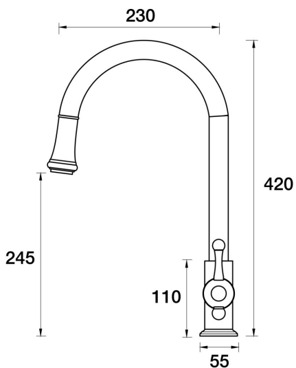
Tudor Sink Pull Out Gooseneck A31.024.1.01 - Chrome
