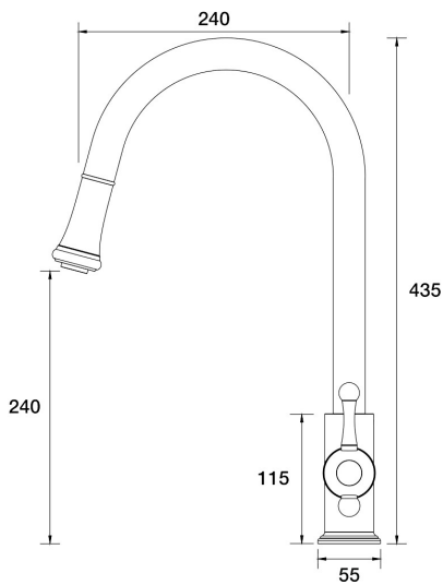
Tudor Sink Pull Out Gooseneck A31.024.1.19 - 23k Brushed Brass Gold
