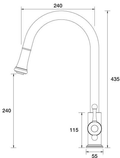
Tudor Sink Pull Out Gooseneck A31.024.1.23 - Gunmetal
