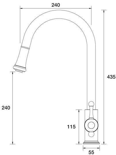
Tudor Sink Pull Out Gooseneck A31.024.1.67 - Vintage Brass
