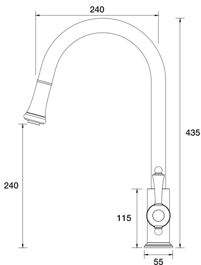
Tudor Sink Pull Out Gooseneck Porcelain Handle A31.024.2.23 - Gunmetal
