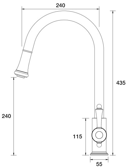
Tudor Sink Pull Out Gooseneck Porcelain Handle A31.024.2.32 - Midnight Black
