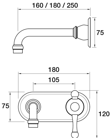
Tudor Wall Mixer Basin Set 200mm outlet Incl. plate Part No. 32.1.34 - Matt Black
