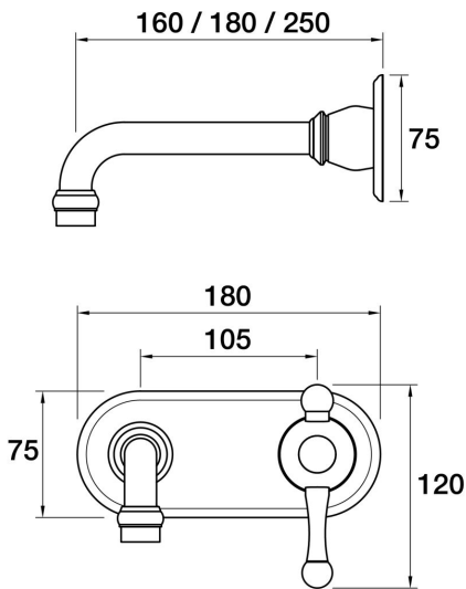
Tudor Wall Mixer Basin Set on plate 160mm A31.032.2.01 - Chrome
