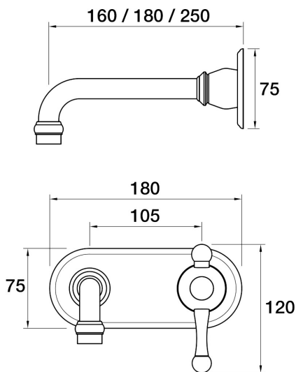
Tudor Wall Mixer Basin Set 160mm outlet Incl. plate Part No. 32.2.47 - Luminick
