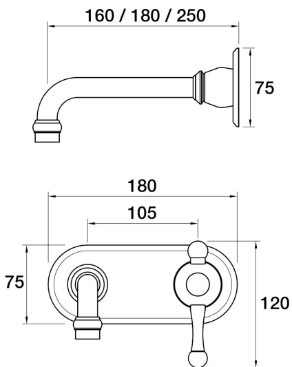
Tudor Wall Mixer Basin Set 160mm outlet Incl. plate PAR-032.2.67 - Vintage Brass
