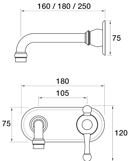
Tudor Wall Mixer Basin Set 250mm outlet Incl. plate PAR032.3.01 - Chrome
