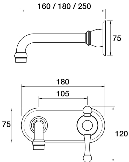
Tudor Wall Mixer Basin Set 250mm outlet Incl. plate Part No. 32.3.21 - Brushed Rose Gold
