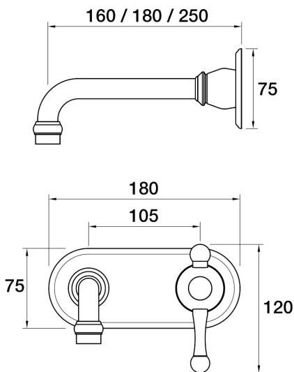
Tudor Wall Mixer Basin Set 250mm outlet Incl. plate Part No. 32.3.24 - Brushed Gunmetal
