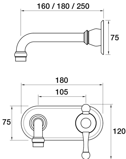
Tudor Wall Mixer Basin Set 250mm outlet Incl. plate PAR-032.3.32 - Midnight Black
