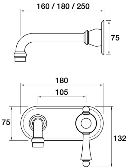
Tudor Wall Mixer Basin Set 200mm outlet incl. plate - porcelain handle A31.032.4.01 - Chrome
