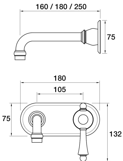
Tudor Wall Mixer Basin Set 200mm outlet incl. plate - porcelain handle A31.032.4.02 - Brushed Chrome
