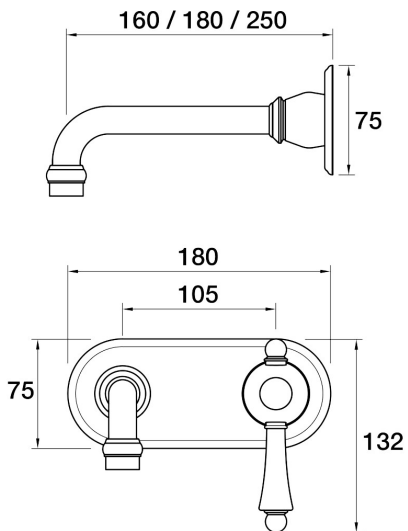
Tudor Wall Mixer Basin Set 160mm outlet incl. plate - porcelain handle A31.032.5.57 - Matt Nickel
