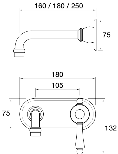
Tudor Wall Mixer Basin Set 250mm outlet incl. plate - porcelain handle A31.032.6.01 - Chrome
