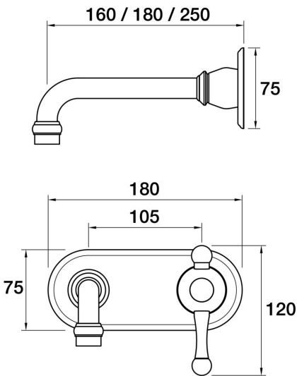
Tudor Wall Bath Mixer Set On Plate 160mm A31.041.1.01 - Chrome
